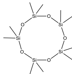
FIGURE 15: Schematic representation of Decamethylcyclopentasiloxane
